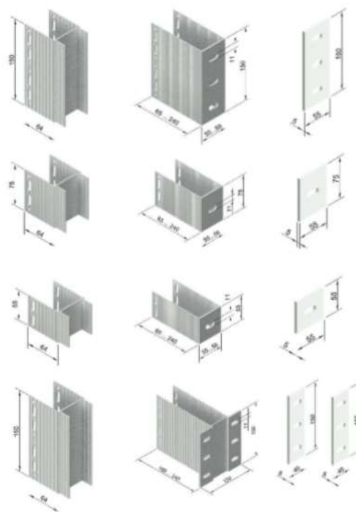
Mounting elements - Brackets – Isolator
