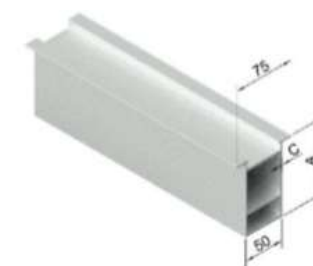
Reinforced profile
